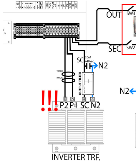
Figure 13. Reversing P1 & P2 cable to get true synchronization
