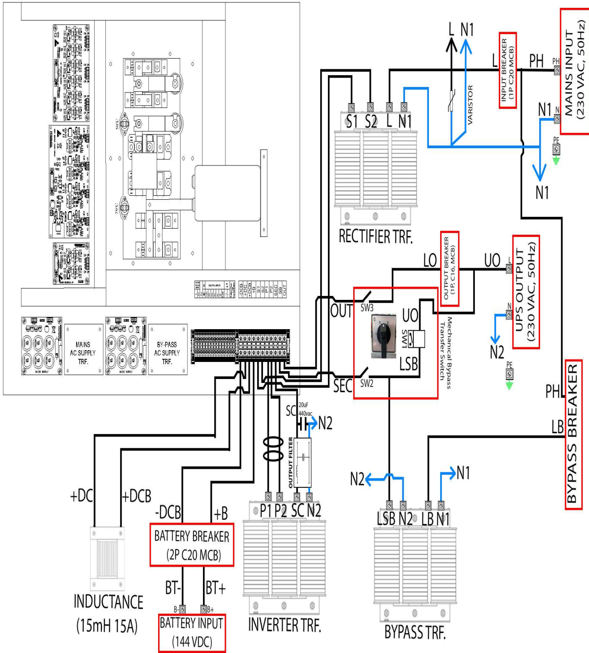
Figure 11. High power cable connections example block diagram of UPS
