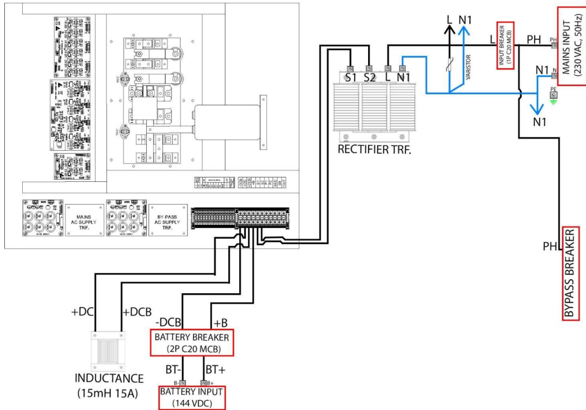
Figure 5. High power cable connections example block diagram of rectifier
