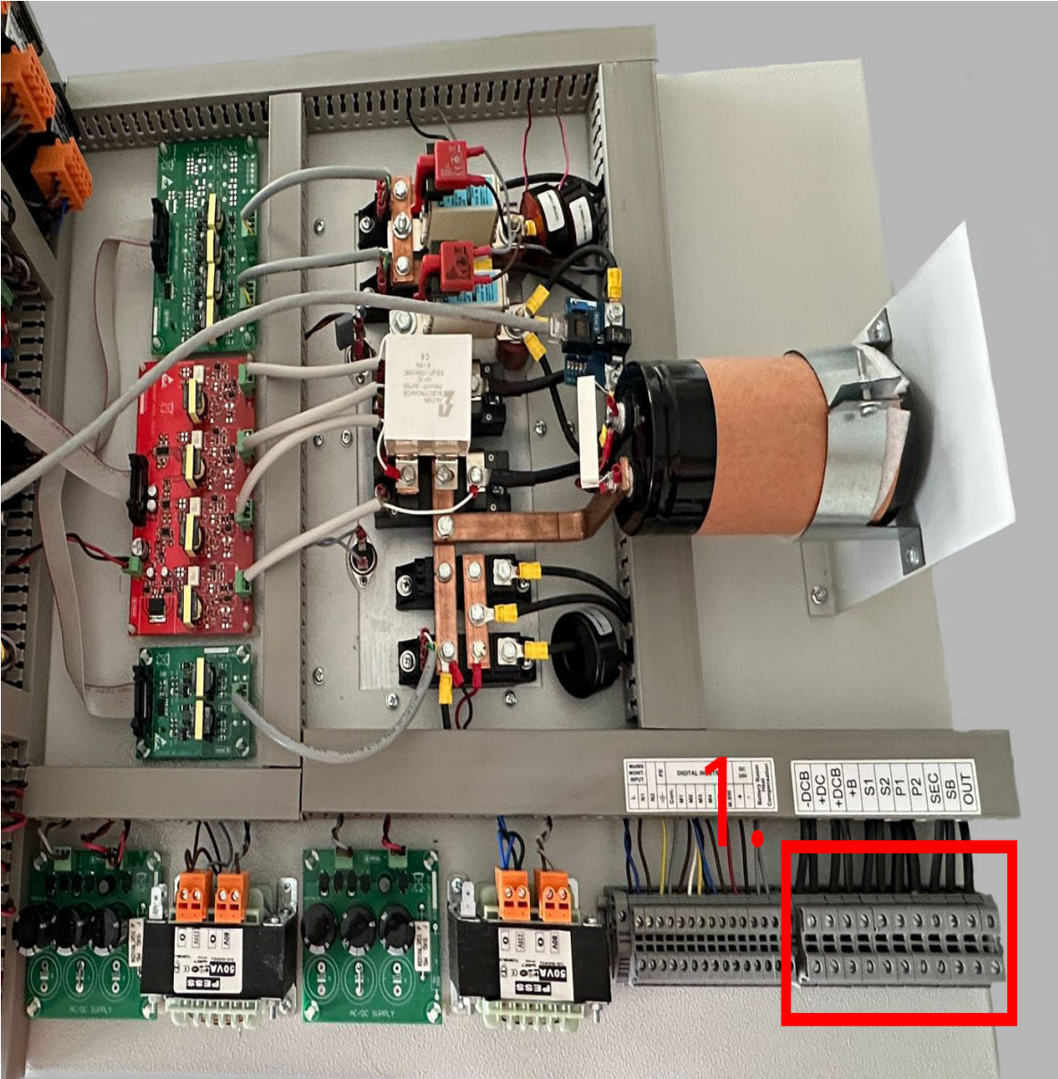
Figure 2. High power cable connection points (port 1)
