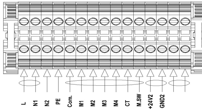
Figure 4. Low signal cable connection points (port 2)
