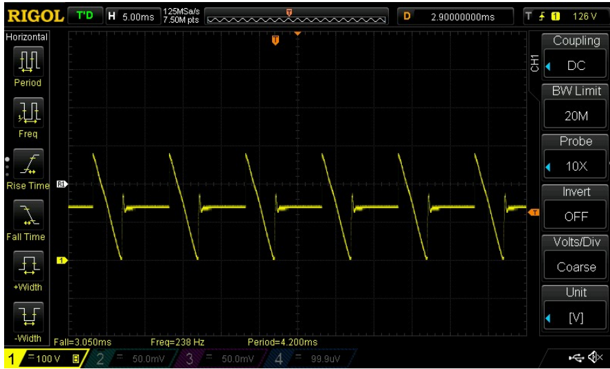
Figure 6. Single phase rectifier true thyristor bus voltage signal.
