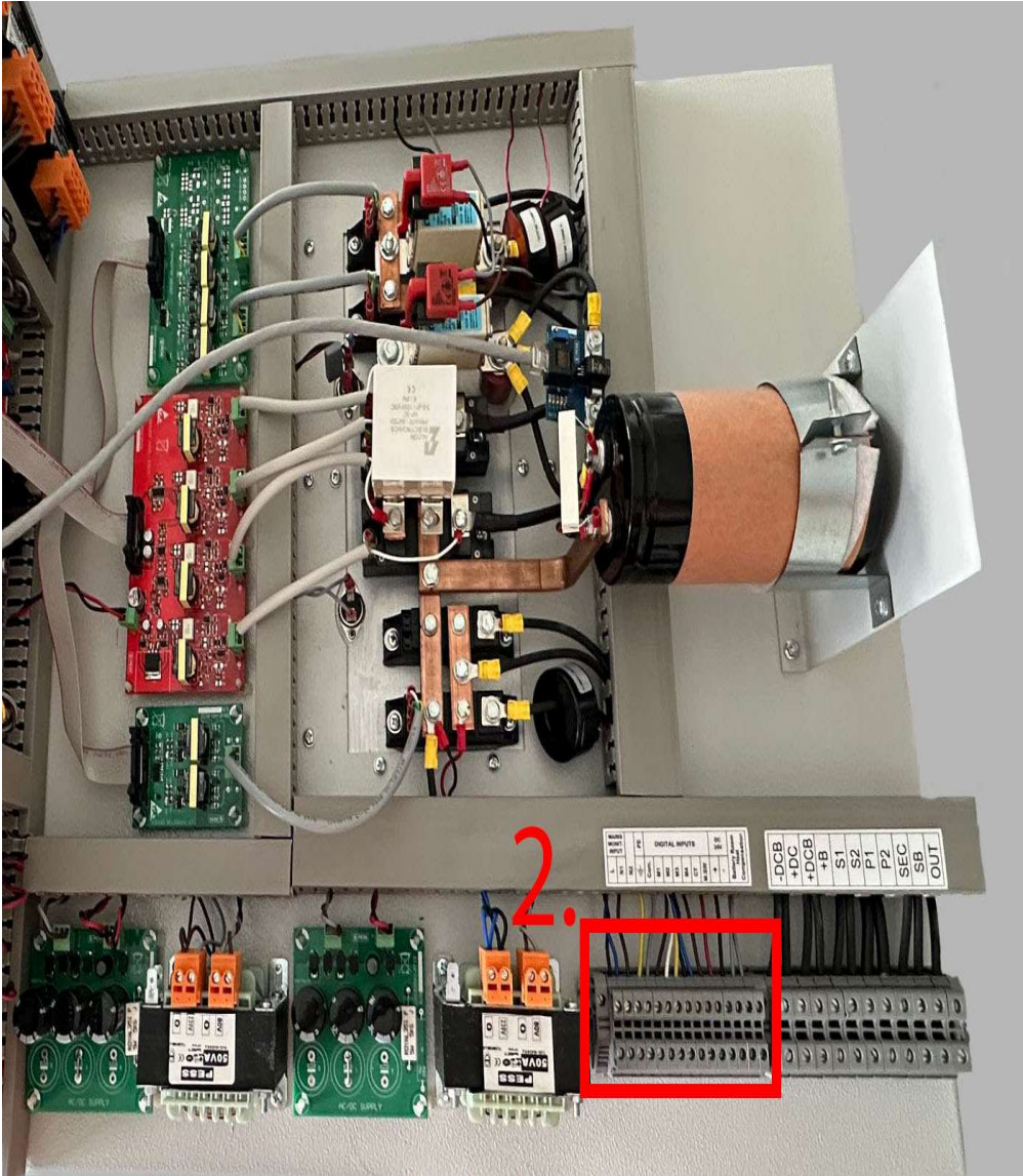
Figure 9. Low signal cable connection points of inverter (port2)
