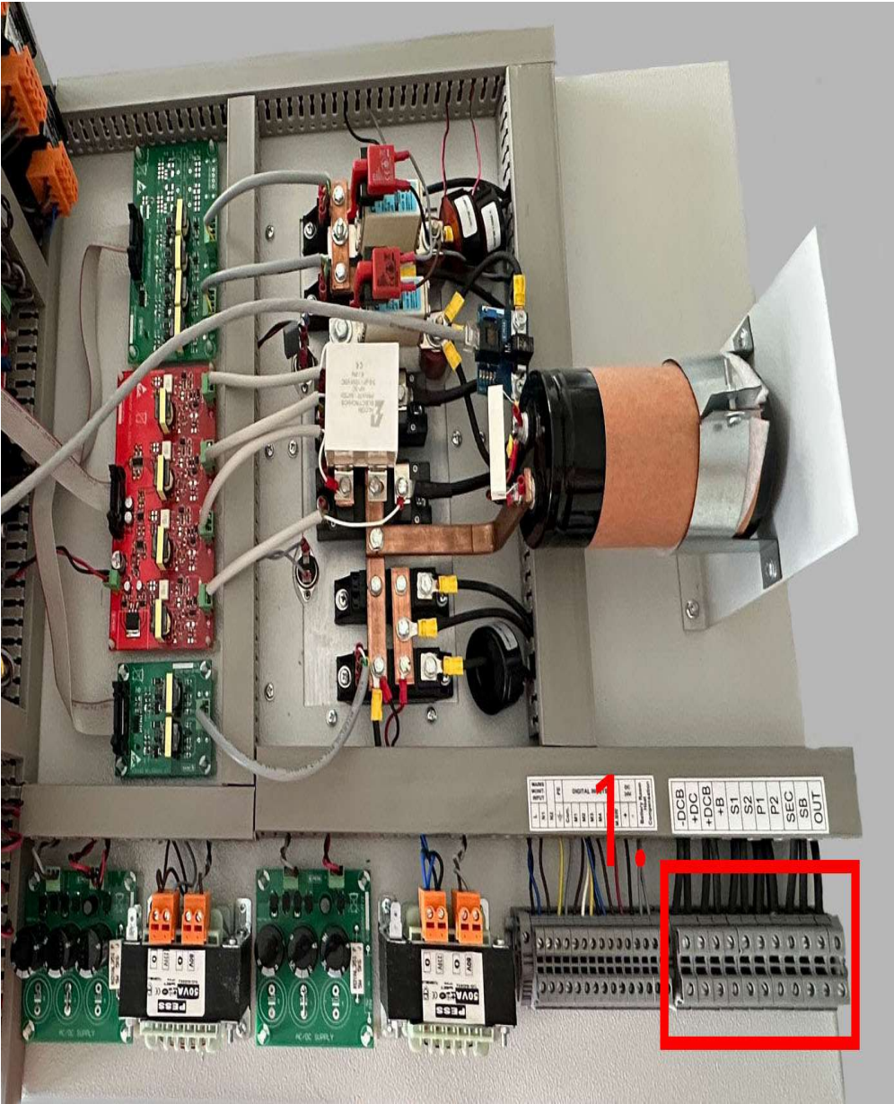
Figure 8. High power cable connection points of inverter (port 1)
