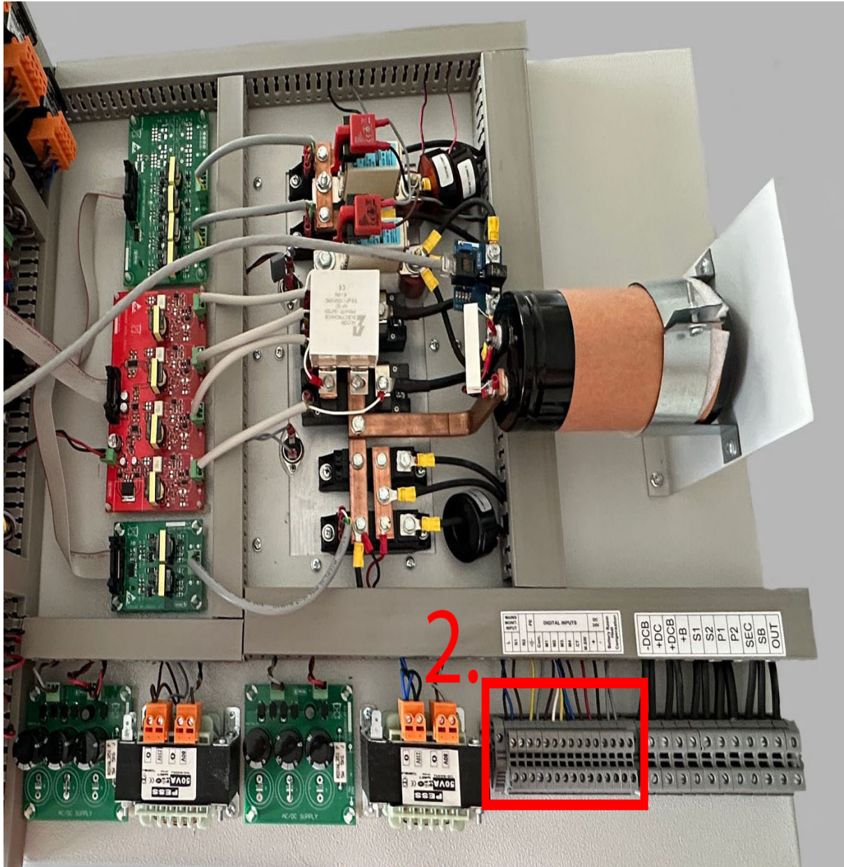
Figure 3. Low signal cable connection points (port 2)
