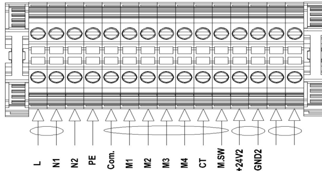
Figure 10. Low signal cable connection points of inverter side as detailed (port2)
