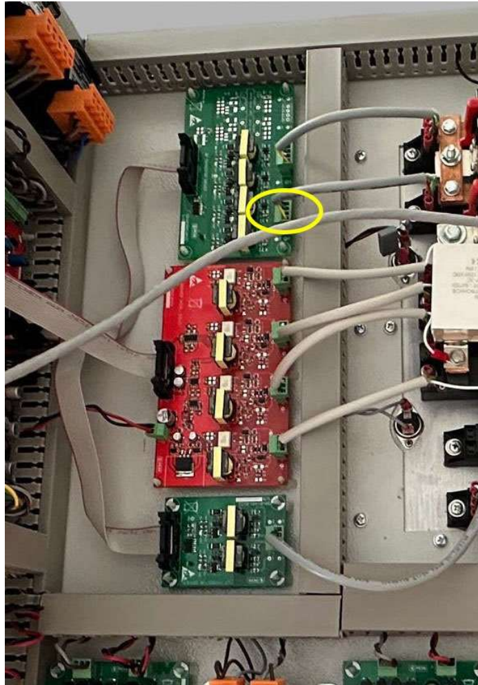
Figure 12. Disconnecting inverter out thyristor to understand true synchronization
