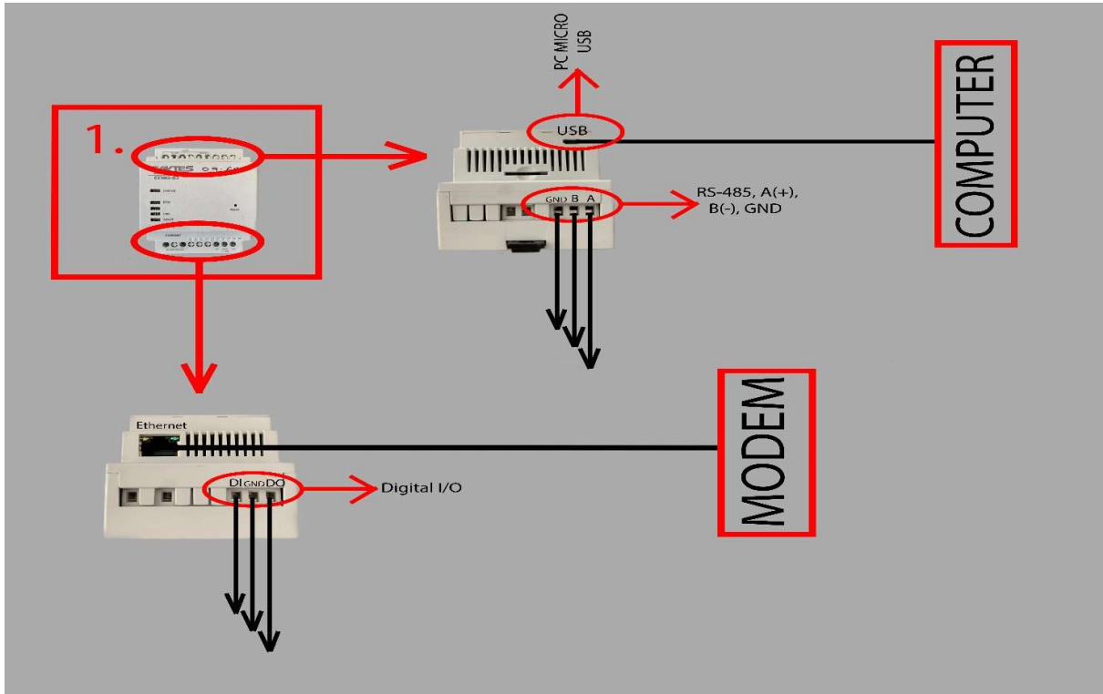
Figure 14. TCP / IP converter connection block diagram.
